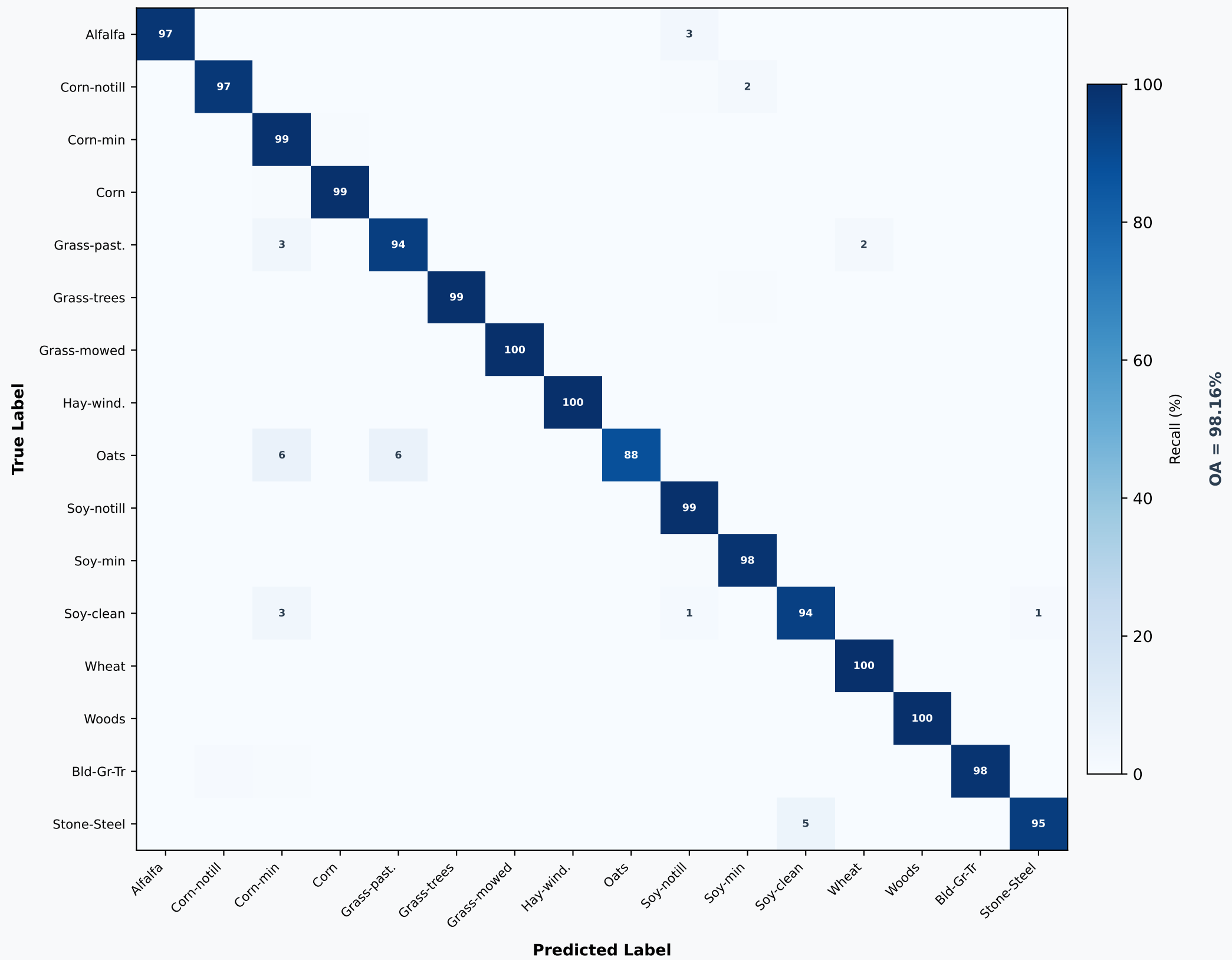
Confusion Matrix — Indian Pines (3D-CNN, All Bands)
